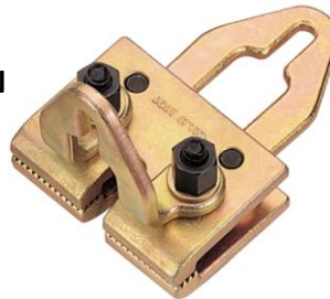
Right Angle Clamp & Yoke 5 ton In-line pull capacity 3 ton right angle pull capacity
